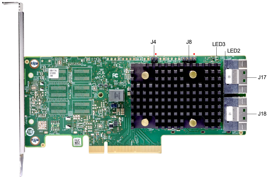
Figure 1: Card Layout of the ThinkSystem 440-16i SAS/SATA PCIe Gen4 12Gb HBA
