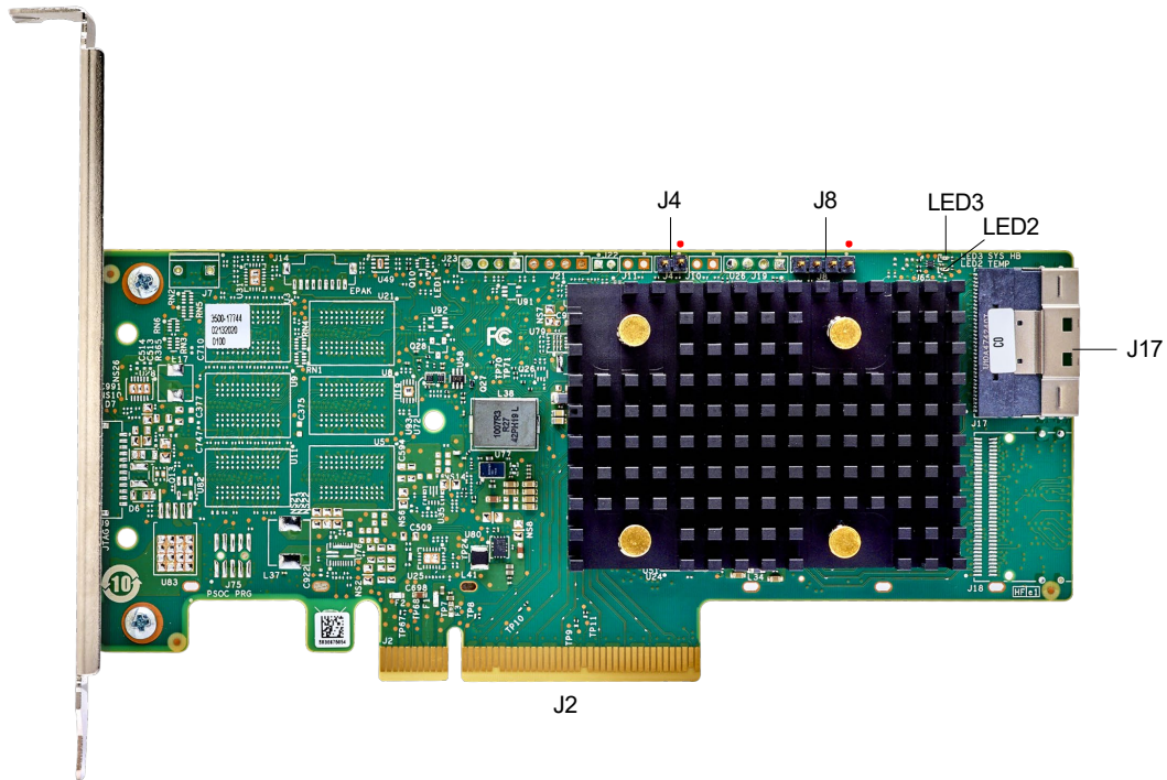
Figure 1: Card Layout of the ThinkSystem 440-8i SAS/SATA PCIe Gen4 12Gb HBA
