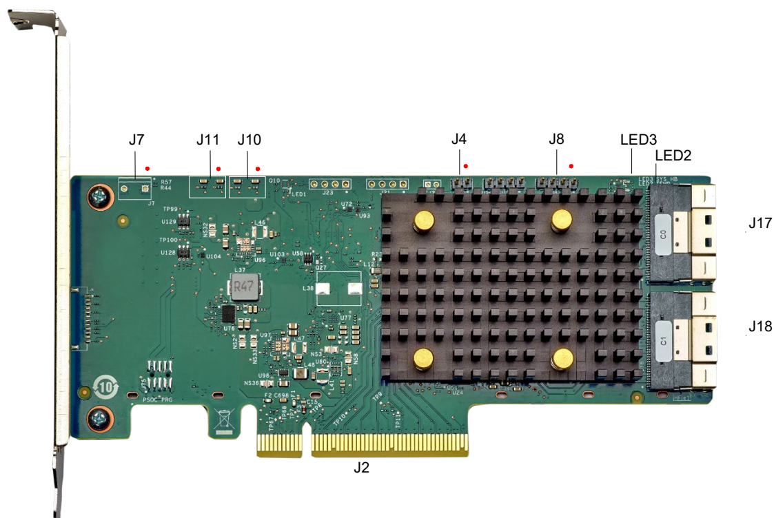
Figure 1: ThinkSystem RAID 540-16i PCIe Gen4 12Gb Adapter
