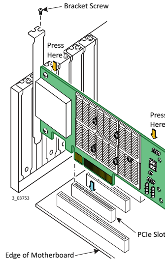
Figure 1 Installing the ThinkSystem 430-16e HBA in a PCIe Slot
