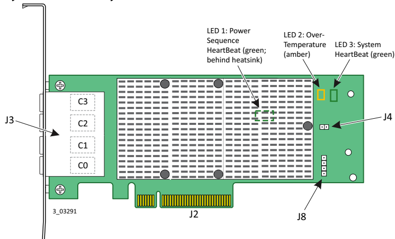
Figure 2 Board Layout of the ThinkSystem 430-16e HBA
