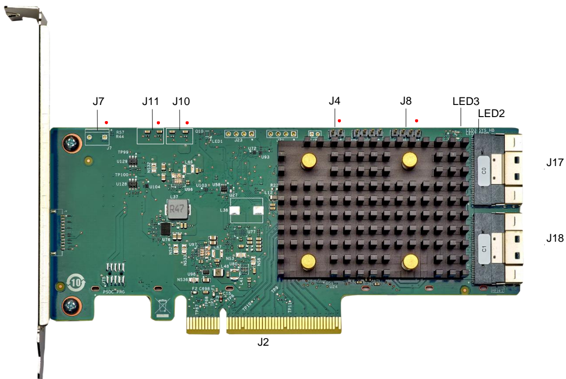
Abbildung 1: ThinkSystem RAID 540-16i PCIe Gen4 12-Gbit-Adapter
