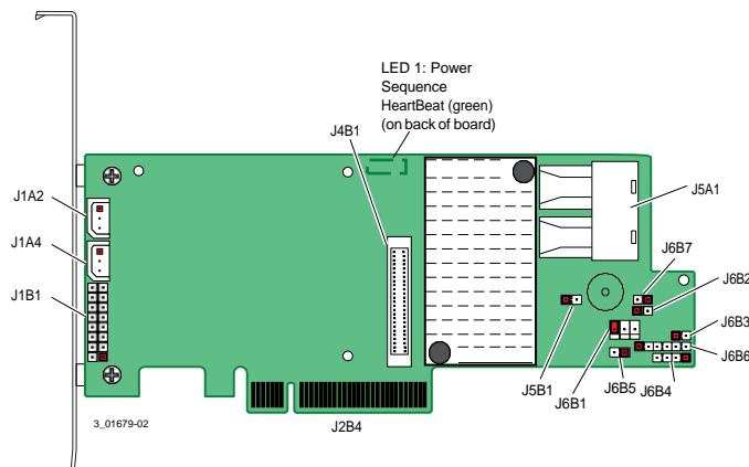
Figure 2 Card Layout for the ThinkSystem RAID 730-8i Adapter
