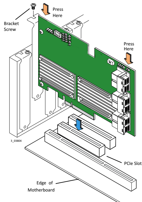
Figure 1 Installing the ThinkSystem RAID 930-24i Adapter in a PCIe Slot
