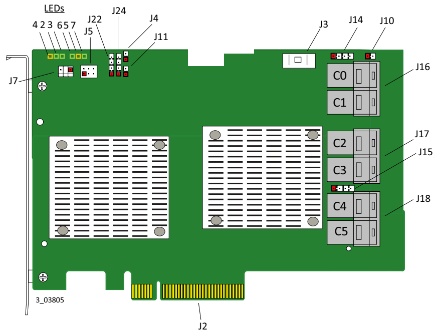
Figure 2 Board Layout for the ThinkSystem RAID 930-24i Adapter
