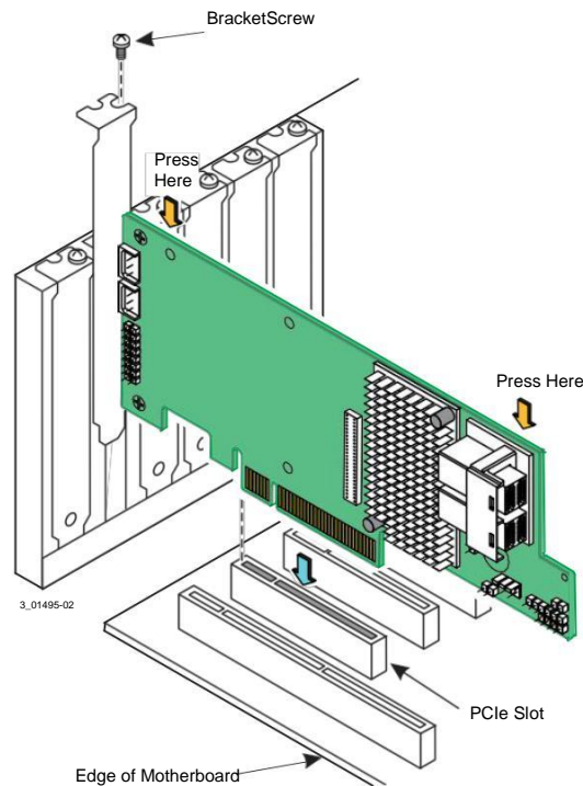
Figure 1 Installing the ThinkSystem RAID 730-8i Adapter in a PCIe Slot
