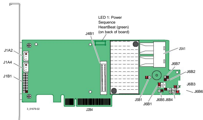
Figure 2 Card Layout for the ThinkSystem RAID 730-8i Adapter
